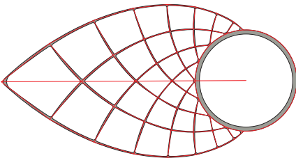
Figure 10: Pattern constructed according the Michell's Theorem for optimal material placement. In the cantilever above, the loading is downward at the point with support connections at the ring. The geometric patterning eliminates bending from the members and resolves forces to 'pure' tension and compression. If the diagram were to be of higher accuracy, the members would be straight lines.
