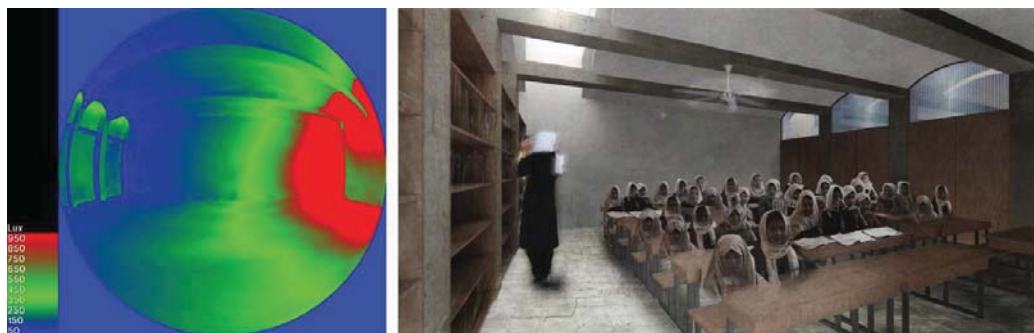
Figure 12: Optimized Afghan vaults create pleasant, daylit classrooms. Source: (Lang and Crofoot 2012)
